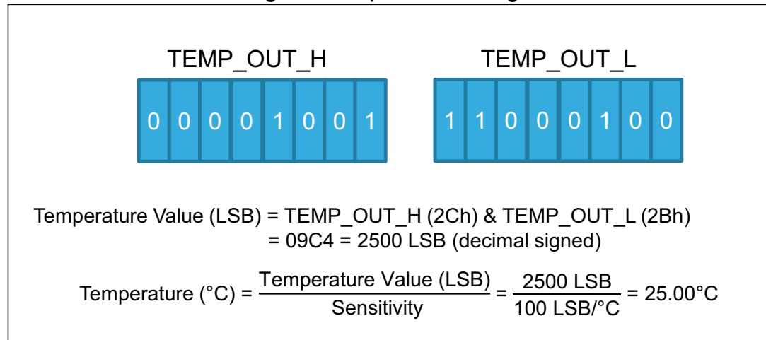
Figure 8. Temperature readings
