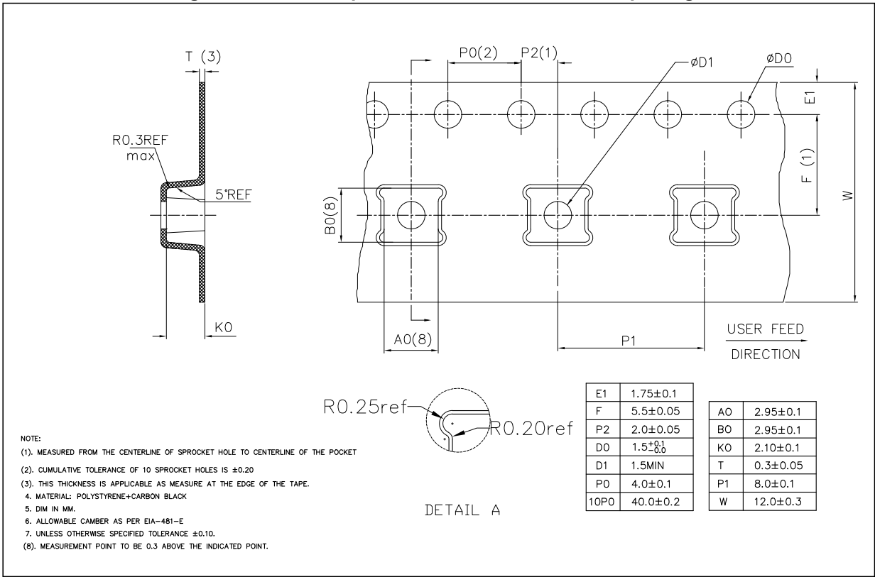
Figure 28. Carrier tape information for CCLGA-10L package
