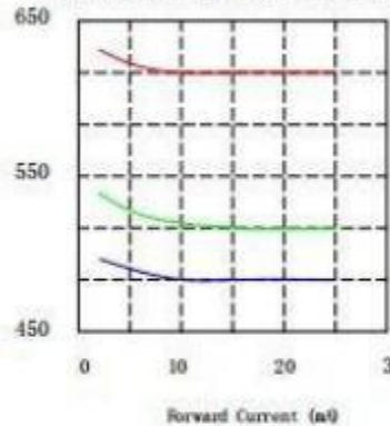
Forward Current vs. Chromaticity ( T_a=25^\circ\text{C} )
