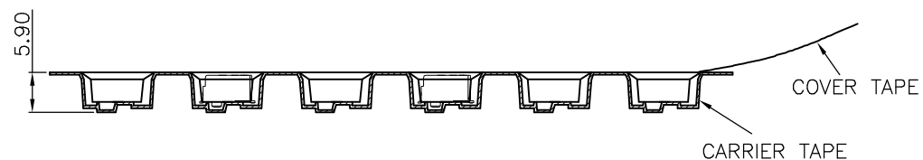
SECTION P-P
