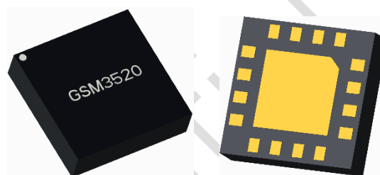
Figure 1. 16 Pad 3 x 3 mm Laminate Package
