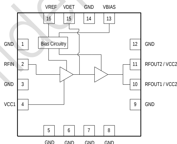
Figure 2. GSM3520 Function Block Diagram
