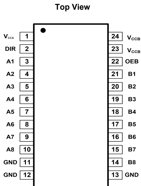
Fig.5-1. GT74LVC8T245: TH (TSSOP24) Package
