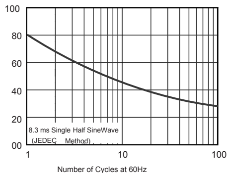
Fig.1 Maximum Non-Repetitive Peak Forward Surge Current
