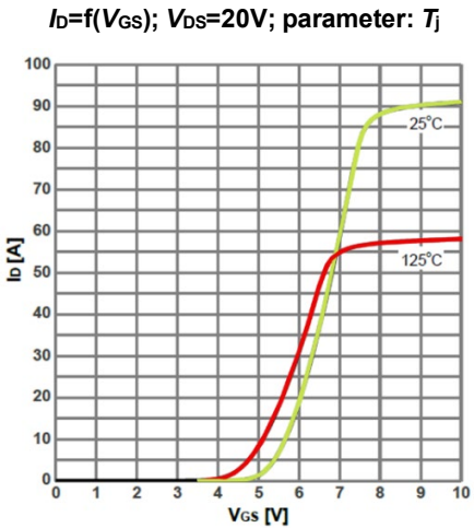
Figure 8. Typ. Transfer characteristics
