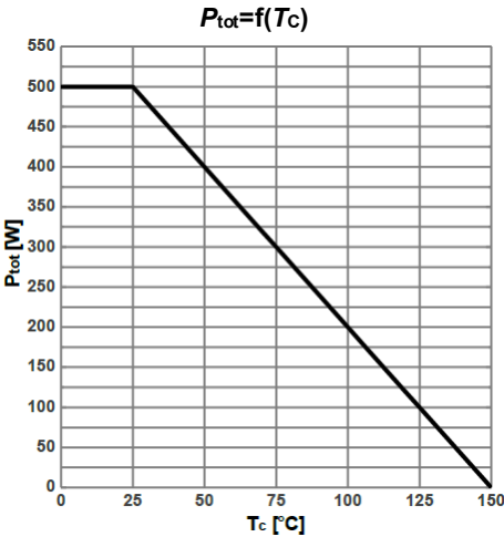
Figure 1. Power dissipation
