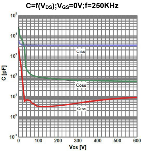
Figure 13. Typ. Capacitances
