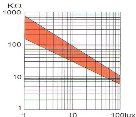
照度-电阻特性 ( Illuminance-resistance characteristics )
