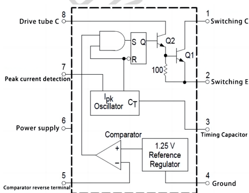
logic diagram
