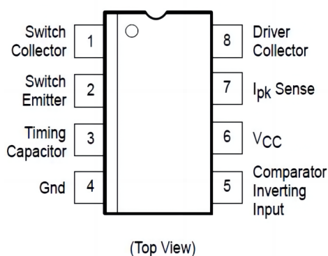
Pin arrangement
