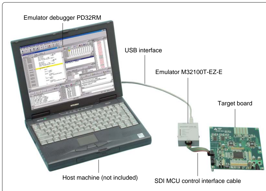
Figure 2.1 System configuration (JTAG connection)
