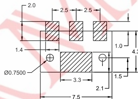
RECOMMENDED PCB LAYOUT TOP VIEW (.XX \pm 0.05)
