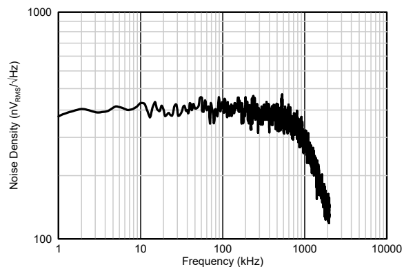
Figure 6-17. Noise Spectral Density vs Frequency
