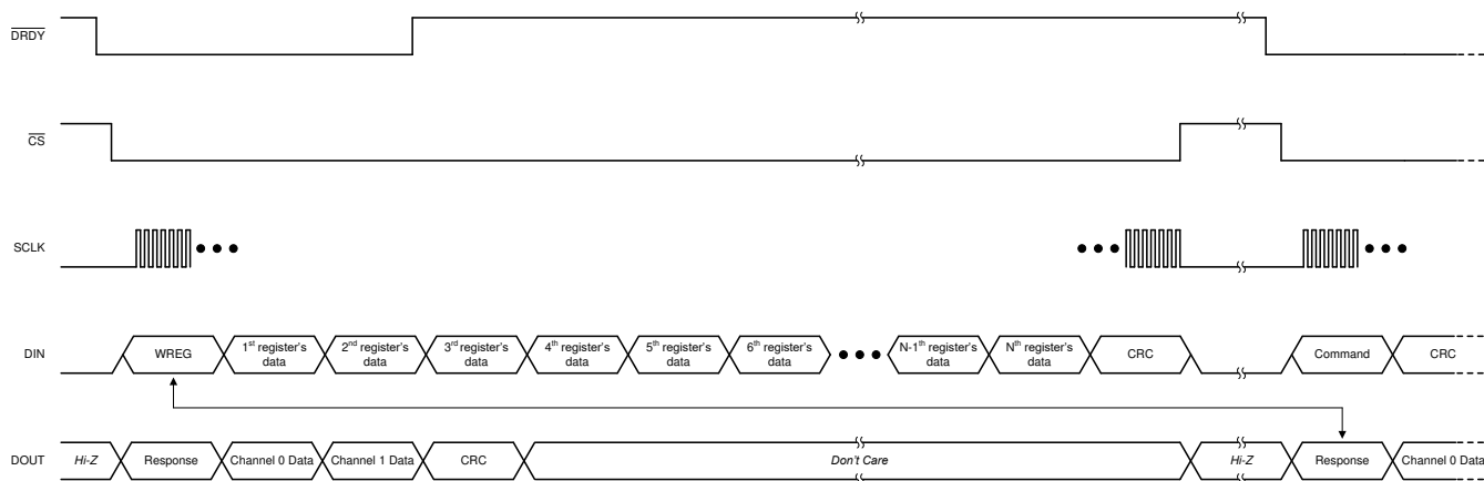
Figure 8-27. Writing Registers
