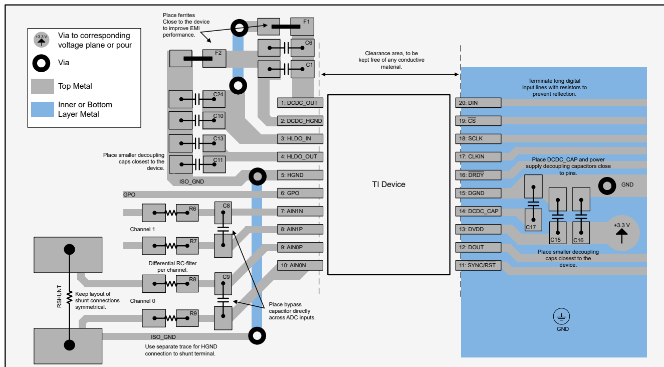
Figure 9-9. Layout Example
