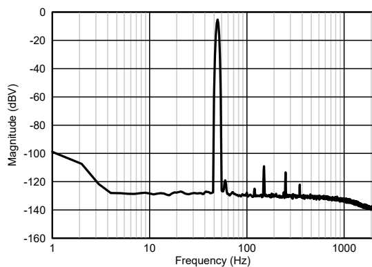
Figure 6-16. Frequency Spectrum With 50-Hz Input Signal
