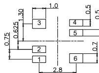
SUGGEST LAYOUT
