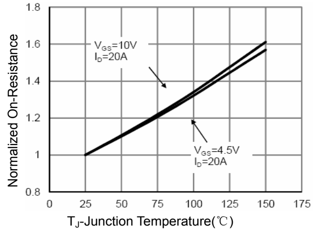
Figure 4 Rdson-Junction Temperature
