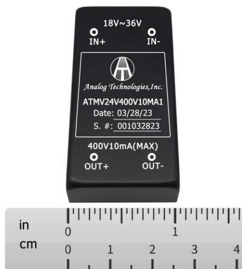
Figure 1. Top View
