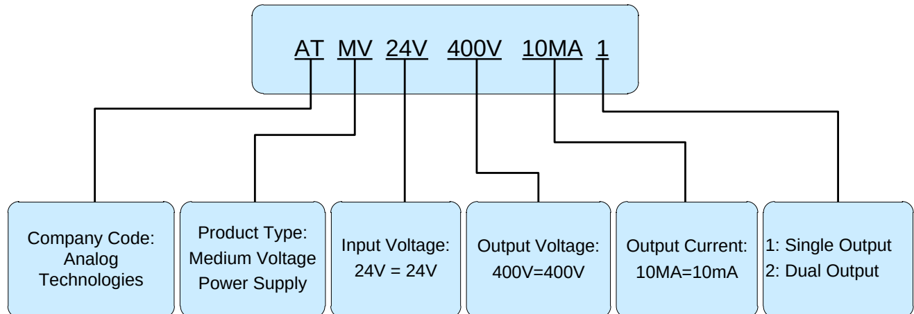
Figure 8. Naming Convention of ATMV24V400V10MA1
