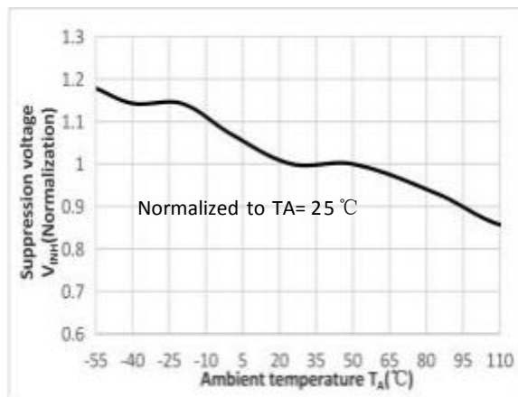
Fig.8 Suppression voltage vs Ambient temperature
