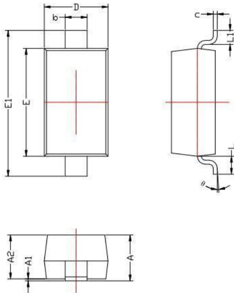
SOD-123 PACKAGE OUTLINE Plastic surface mounted package
