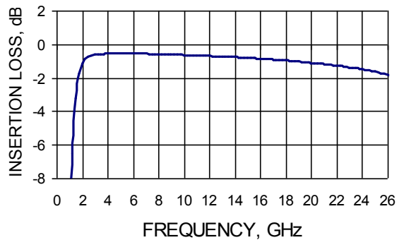
INSERTION LOSS vs FREQUENCY MA4SW210B-1
