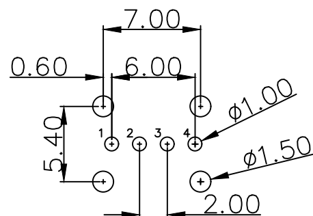
RECOMMEND PCB LAYOUT(±0.05)
