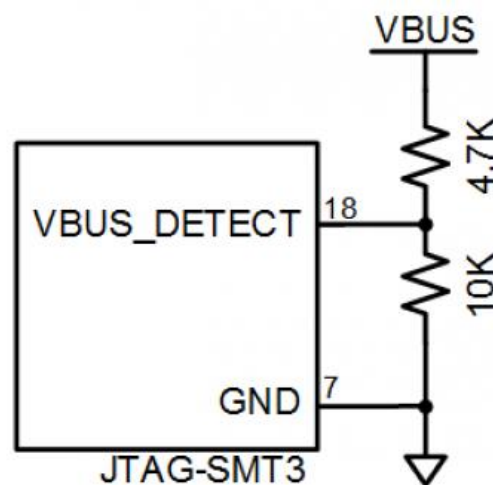
Figure 3. Connecting VBUS to the VBUS_DETECT pin.
