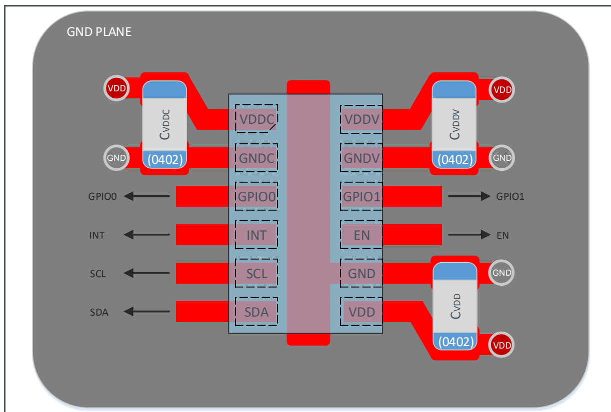
Figure 122: PCB Layout Recommendation
