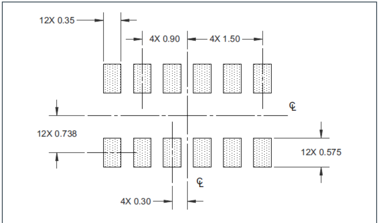
Figure 123: PCB Pad Layout
