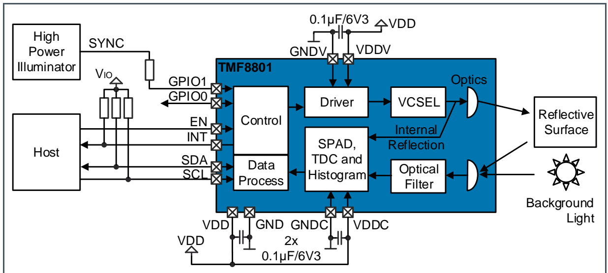
Figure 120: TMF8801 Application Schematic
