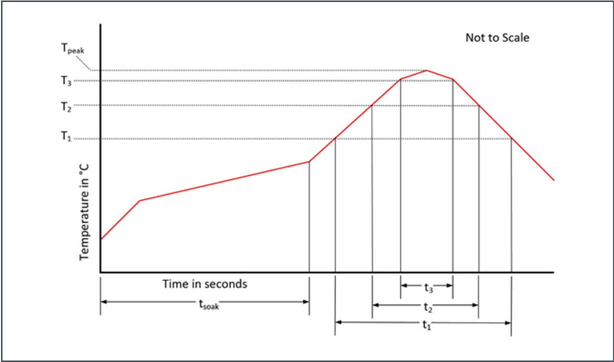
Figure 126: Solder Reflow Profile Graph
