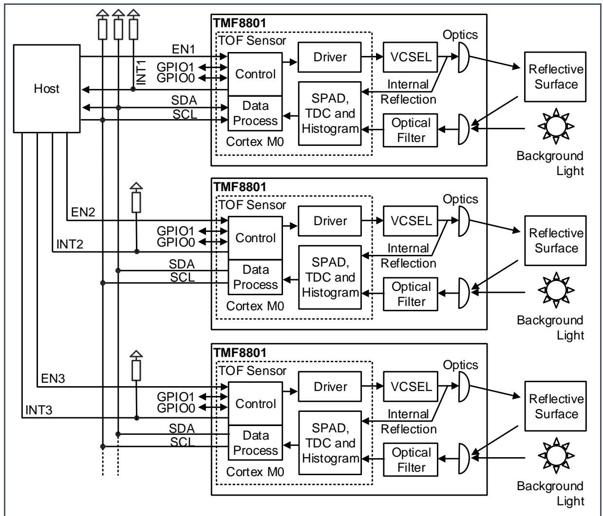
Figure 121: Sharing a Single I 2 C Bus for Operating Several TMF8801s
