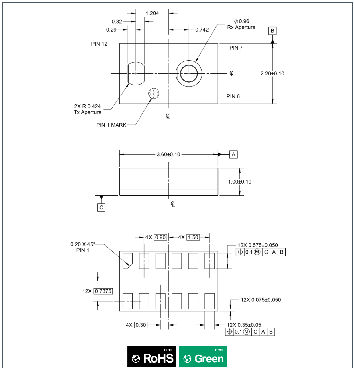
Figure 124: Package Drawing
