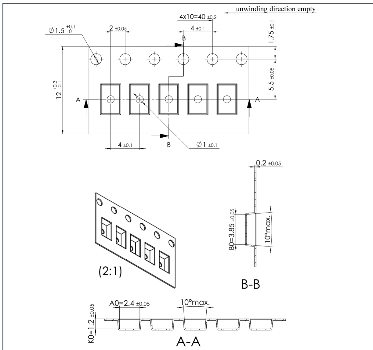
Figure 125: Tape and Reel Drawing
