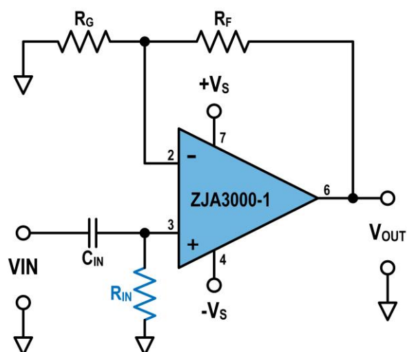
Figure 40. Creating an Input Bias Current Return Path
