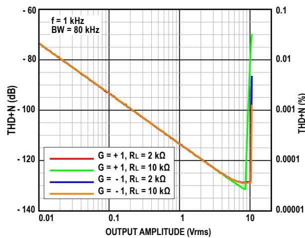
Figure 31. THD+N vs. Amplitude
