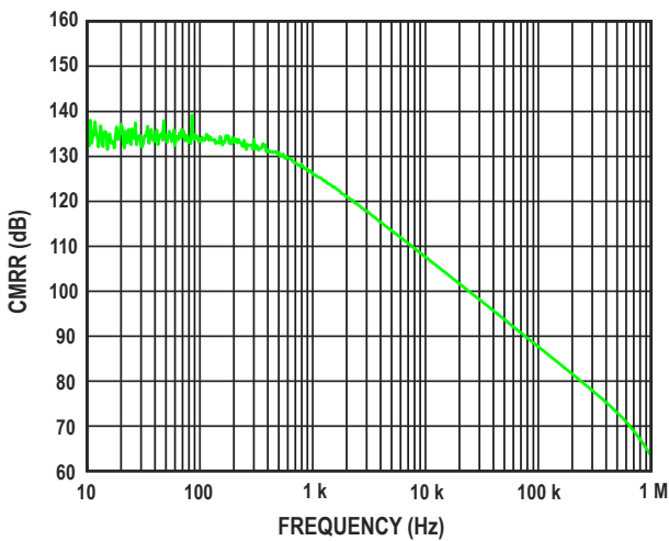
Figure 24. Common Mode Rejection Ratio (CMRR) vs. Frequency
