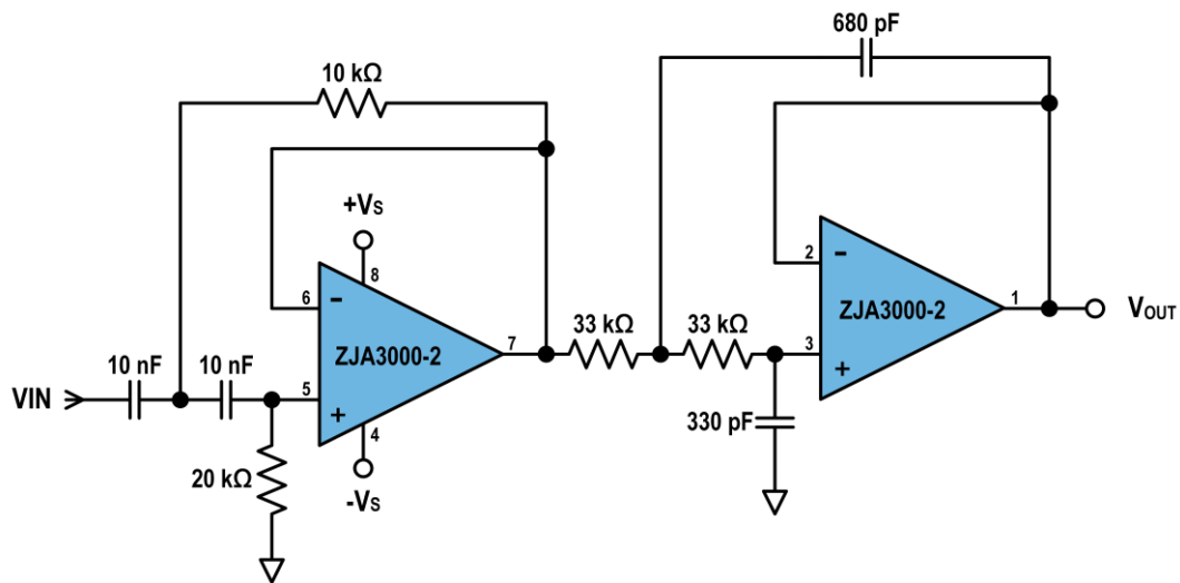
Figure 41. Using ZJA3000-2 to Build a 2-stage Band-pass KRC Filter
