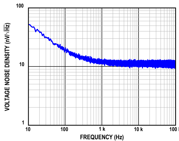
Figure 33. Voltage Noise Density vs. Frequency
