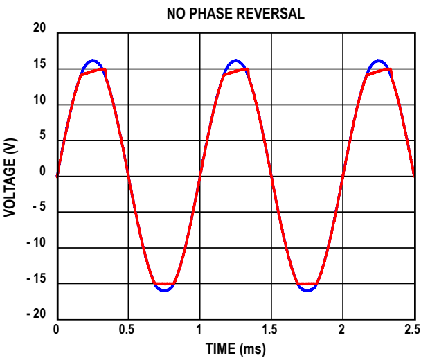
Figure 38. ZJA3000 Has No Output Phase Reversal
