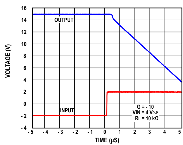
Figure 21. Negative Overload Recovery
