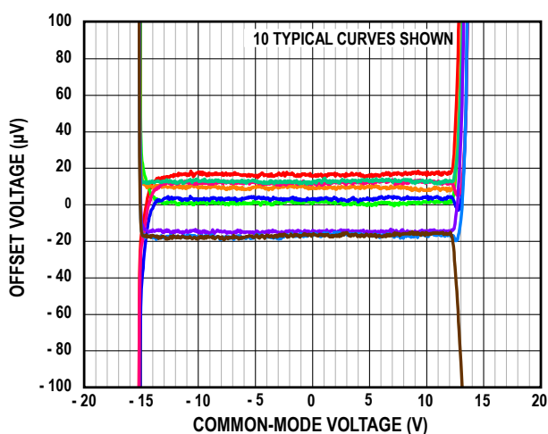
Figure 10. Offset Voltage vs. Input Common-Mode Voltage
