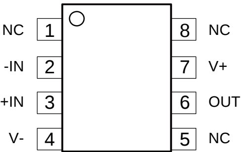
Figure 1. ZJA3000-1 Pin Configuration (8-lead SOIC and MSOP)
