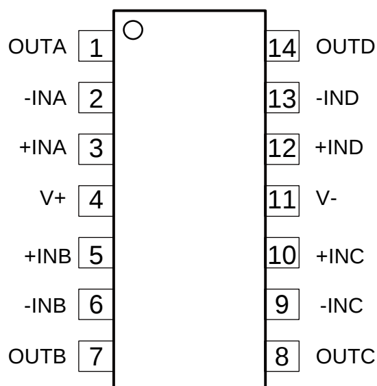
Figure 3. ZJA3000-4 Pin Configuration (14-lead SOIC and TSSOP)
