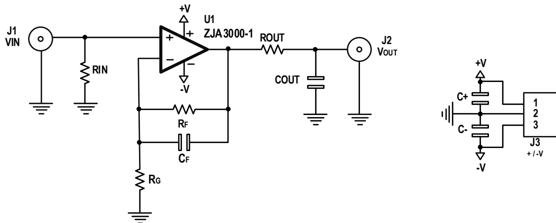
Figure 42. Op Amp Schematic for Non-inverting Configuration
