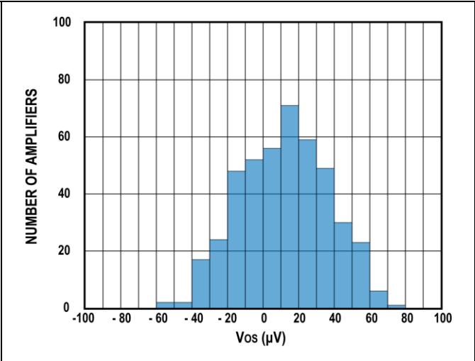
Figure 5. Input Offset Voltage Distribution at -40 °C, SOIC-8 Package
