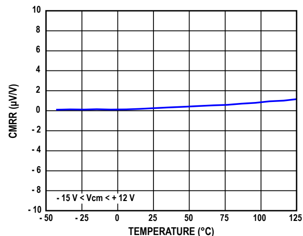
Figure 17. Common Mode Rejection Ratio (CMRR) vs. Temperature
