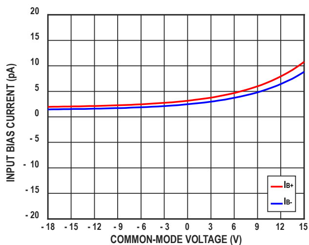
Figure 11. Input Current vs. Input Common-Mode Voltage ( V_{SY} = \pm 18\text{ V} )
