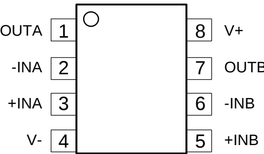
Figure 2. ZJA3000-2 Pin Configuration (8-lead SOIC and MSOP)
