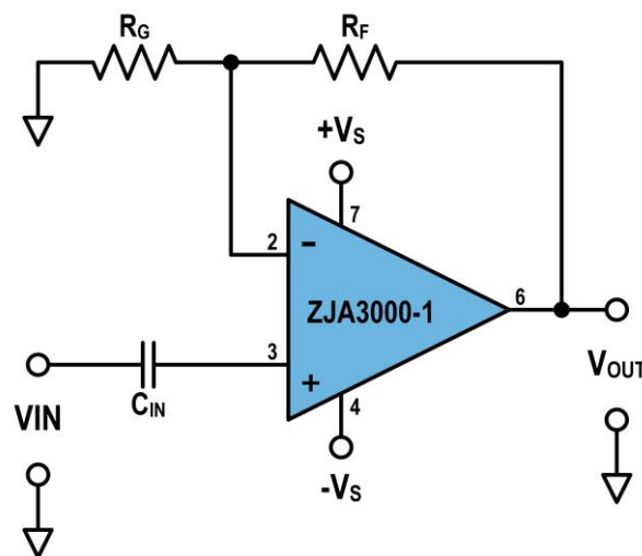
Figure 39. Incorrect AC-Coupled Op Amp Circuit
