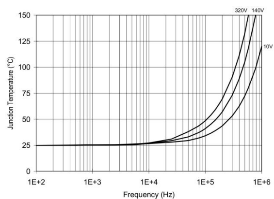
Figure 32. DOT2110S/DOT2113S TJ vs. Frequency(IRFBC20) RGATE = 33 \Omega , VCC = 15V
