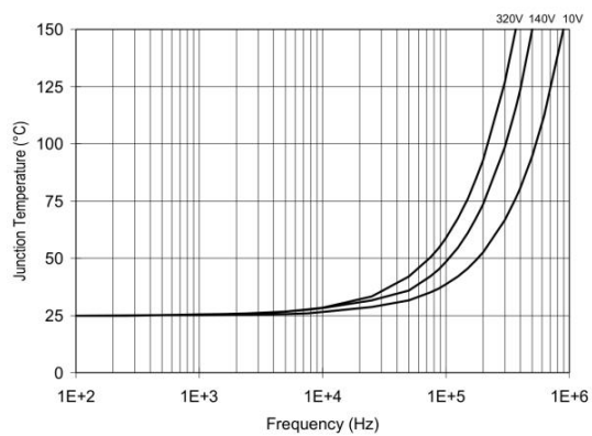
Figure 35. DOT2110S/DOT2113S T_J vs. Frequency (IRFPE50) R_{GATE} = 10\Omega , V_{CC} = 15V
