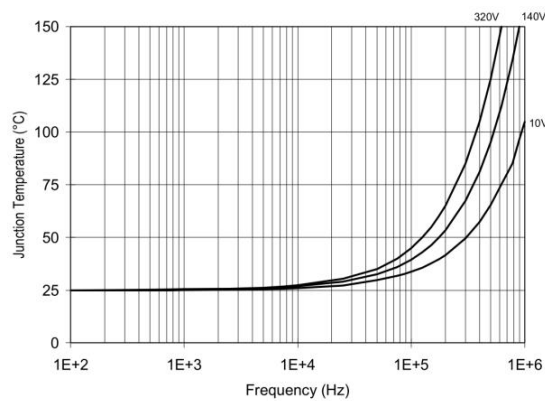
Figure 29. DOT2110/DOT2113 TJ vs. Frequency(IRFBC30) RGATE = 22 \Omega , VCC = 15V
