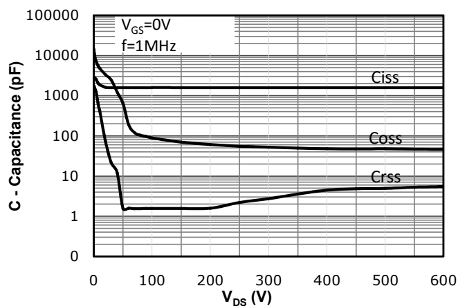
Fig 11: Capacitance Characteristics
