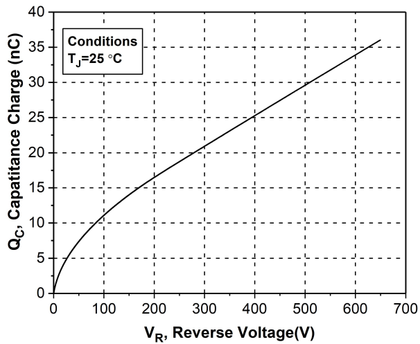
Figure 5. Capacitance Charge Vs. Reverse Voltage
