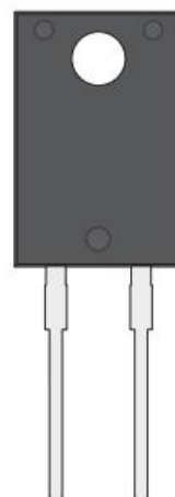
TO-220F-2L mechanical data
