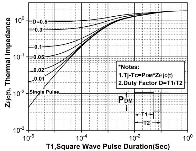
Figure 8. Transient Thermal Response Curve(Junction-to-Case)
