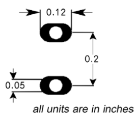
TO-220F-2L
