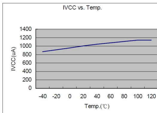
Ivcc vs. Temp.
