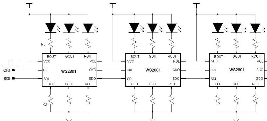
Fig4, The typical application circuit of WS2801
