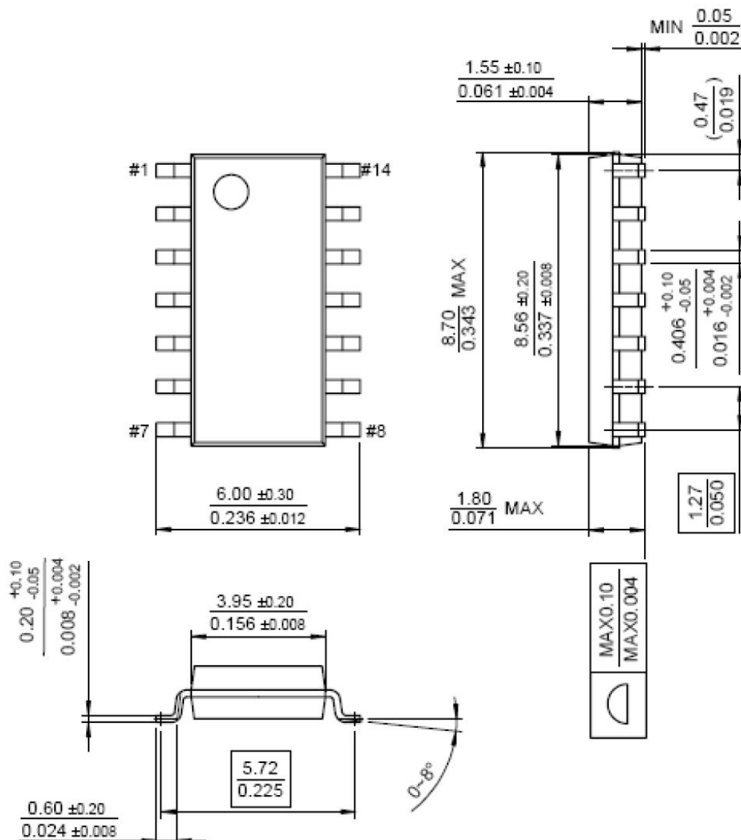
SOP-14 Package (Unit: mm)
