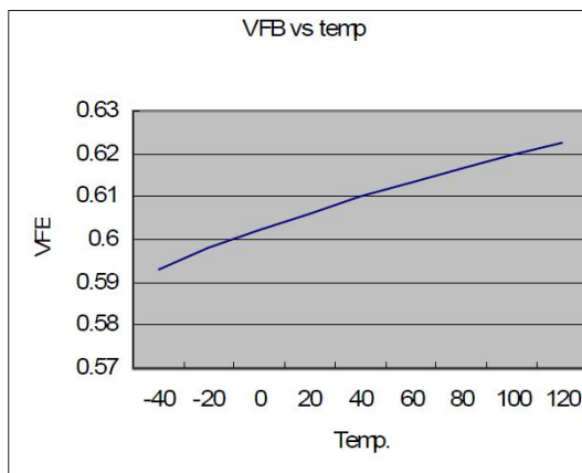
Feed back voltage vs. temp.
