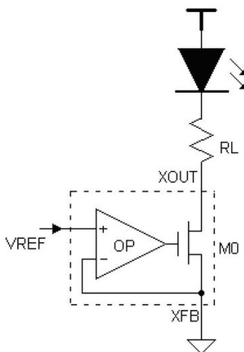
Fig7, The schematic of constant voltage driving mode
