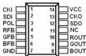
Fig1. SOP-14 package
