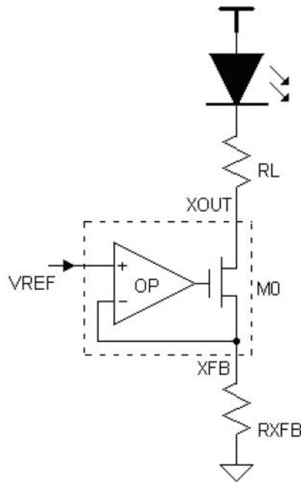
Fig6, The schematic of constant current drive
