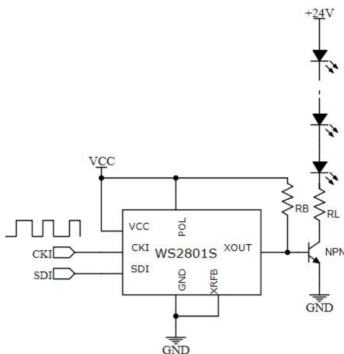
Fig8, Constant Voltage Driving with External Power Switches.
