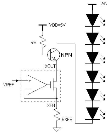
Fig9, Constant current drive with external switches
