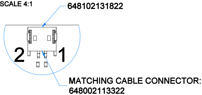
DETAIL B SCALE 4:1
