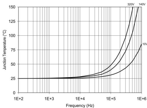
Figure 33. DOT2110S/DOT2113S TJ vs. Frequency(IRFBC30) RGATE = 22Ω, VCC = 15V
