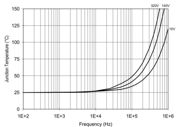
Figure 32. DOT2110S/DOT2113S TJ vs. Frequency(IRFBC20) RGATE = 33Ω, VCC = 15V
