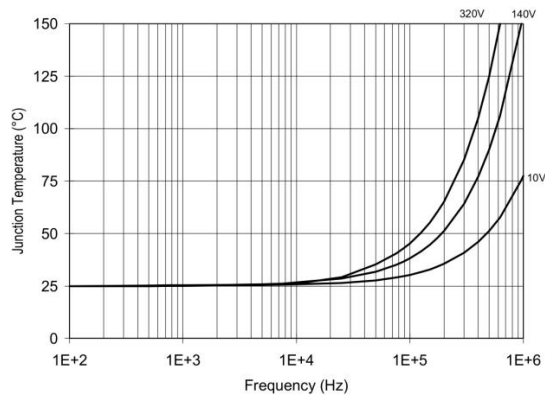
Figure 30. DOT2110/DOT2113 TJ vs. Frequency(IRFBC40) RGATE = 15Ω, VCC = 15V
