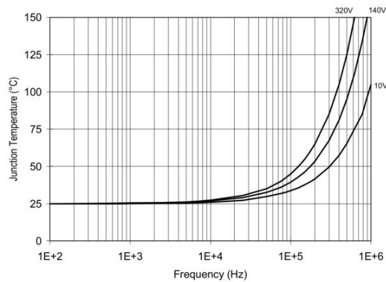
Figure 29. DOT2110/DOT2113 TJ vs. Frequency(IRFBC30) RGATE = 22Ω, VCC = 15V
