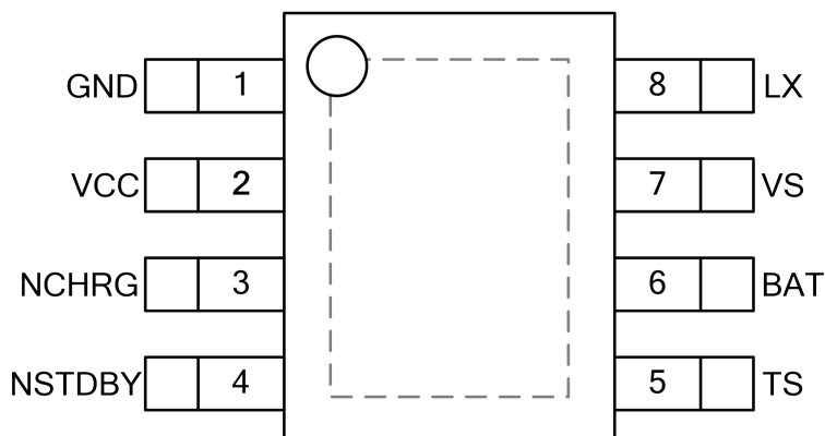
Figure 4. SLM6500 Package
