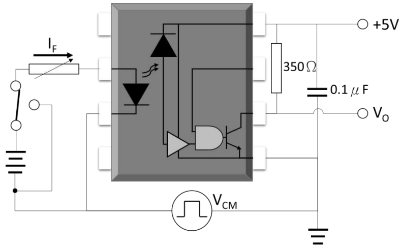
Fig.25 Test Circuits for Common Mode Transient Immunity
