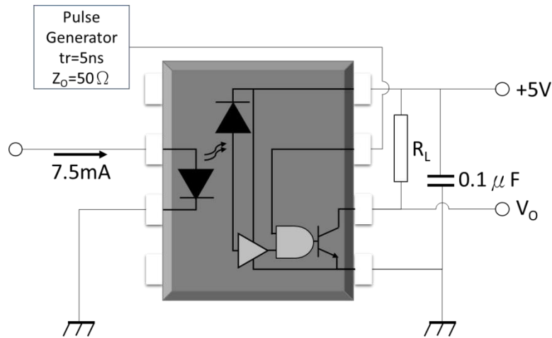
Fig.25 Test Circuits for TEHL, TELH
