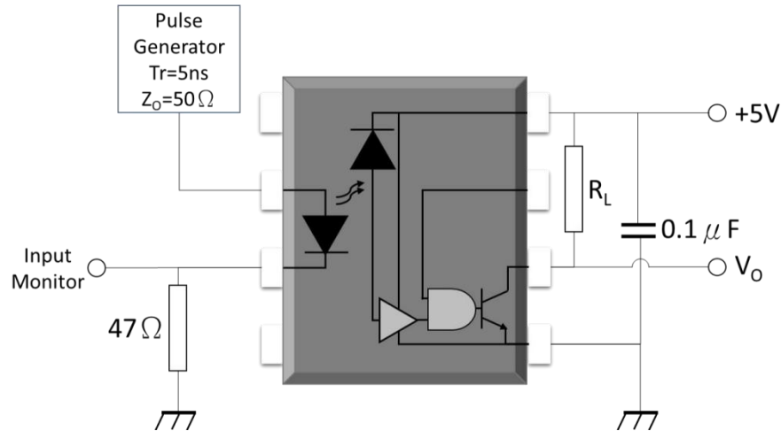
Fig.23 Test Circuits for TPHL, TPLH, tr, tf
