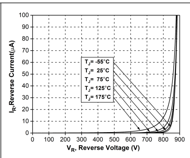
Figure 2. Reverse Characteristics
