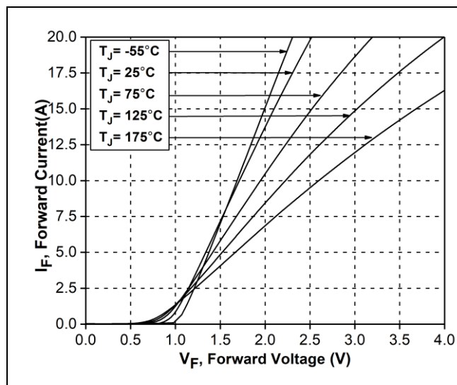
Figure 1. Forward Characteristics
