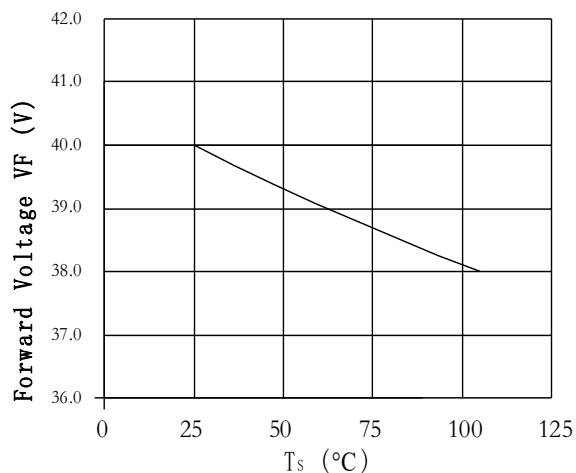
Case Temperature vs. Forward Voltage 结点温度与正向电压曲线图 IF=450mA
