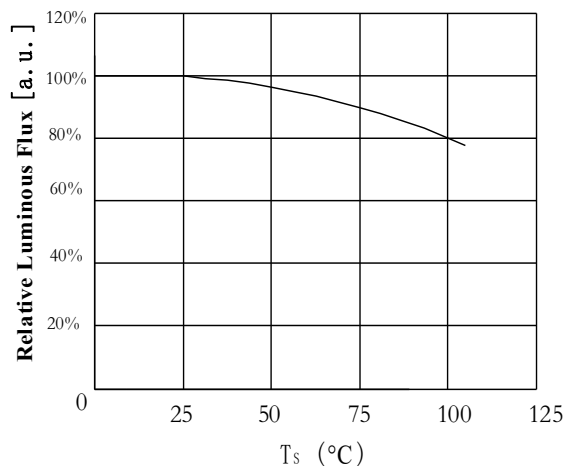
Case Temperature vs. Relative Luminous Flux 结点温度与相对流明曲线图 IF=450mA
