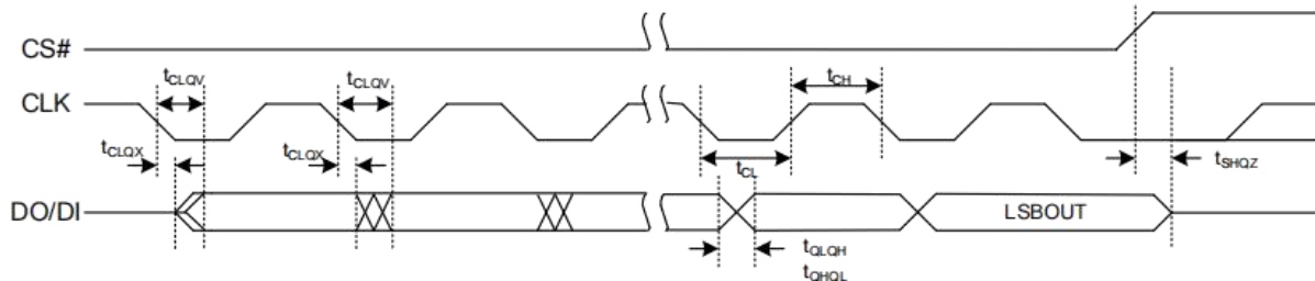
Figure 10.4 Serial Output Timing
