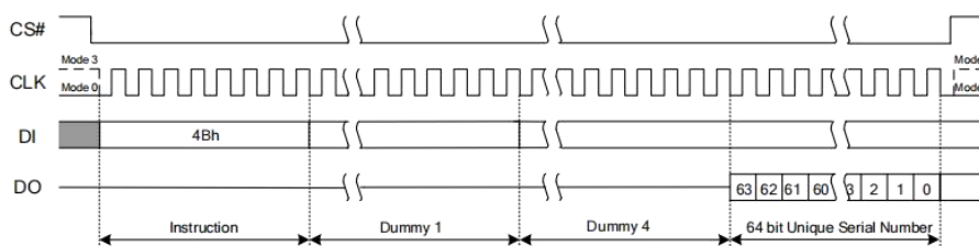
Figure 9.38 Read unique ID Number Instruction
