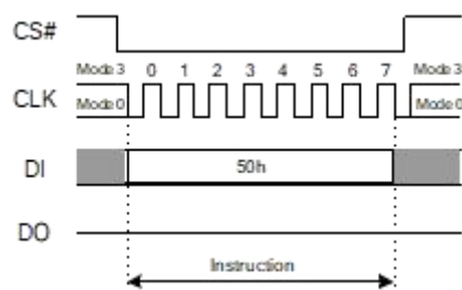
Figure 9.3 Write Enable for Volatile Status Register Instruction
