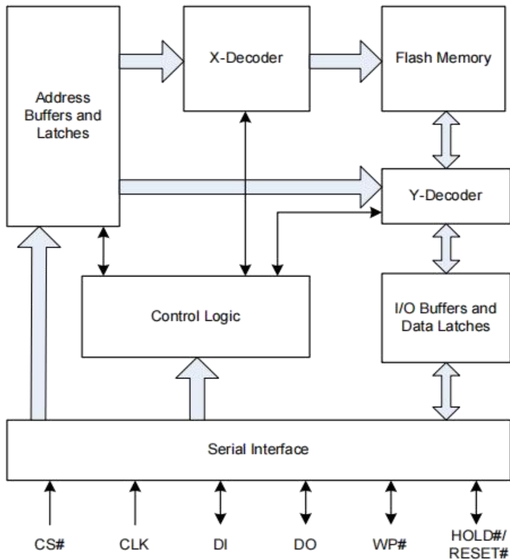
Figure 4.1 Block Diagram
