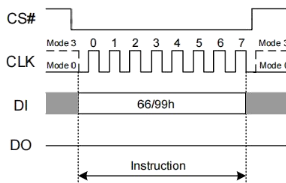
Figure 9.26 Software Reset Instruction
