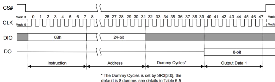
Figure 9.14a Fast Read Instruction
