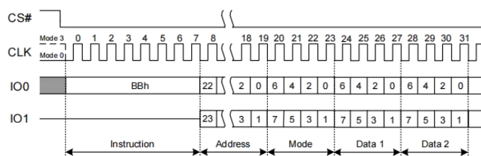
Figure 9.17 Fast Read Dual I/O Instruction (Initial command or previous M5-4≠10)
