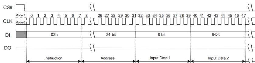
Figure 9.9a Page Program Instruction
