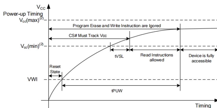
Figure 10.1 Power-up Timing
