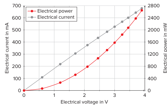
Electrical specifications
