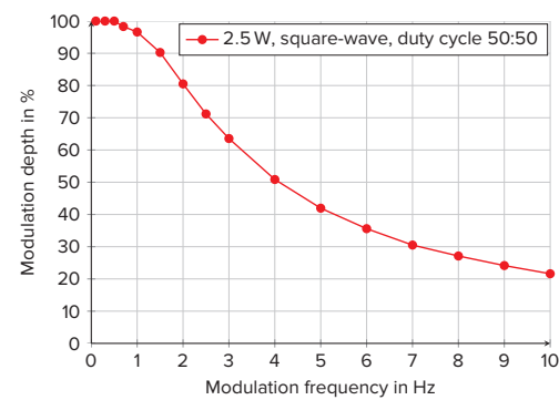
Modulation depth
