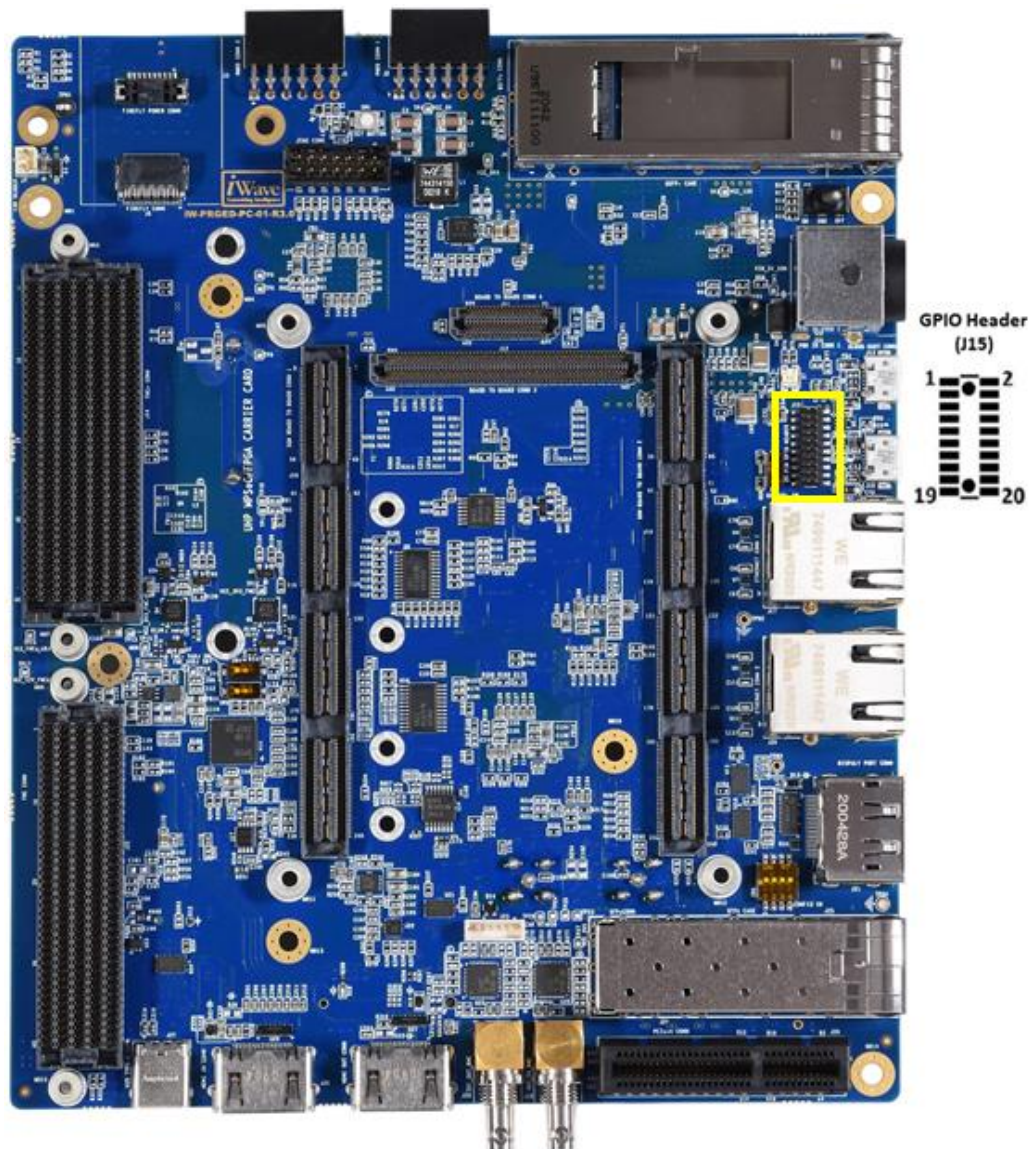
Figure 30: GPIO Header
