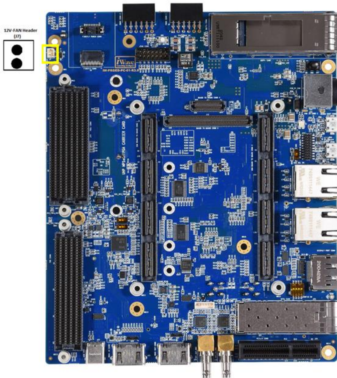
Figure 34: 12V-Fan Header
