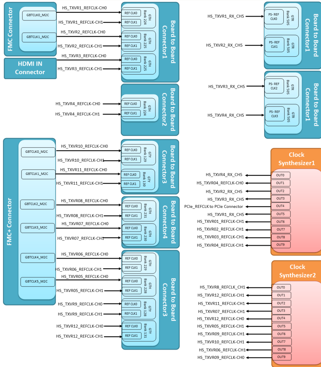
Figure 27: Clock Tree
