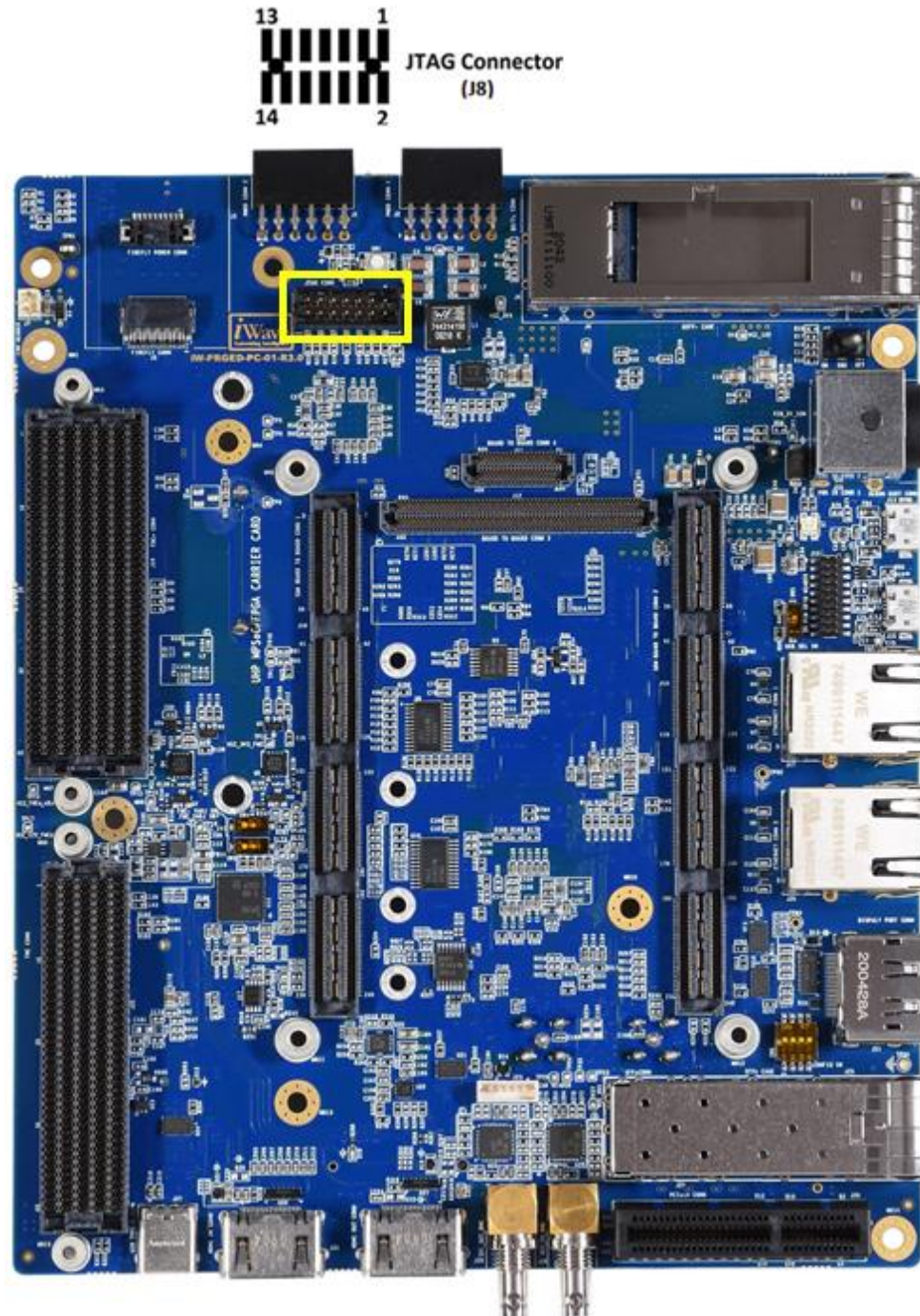
Figure 28: JTAG Connector
