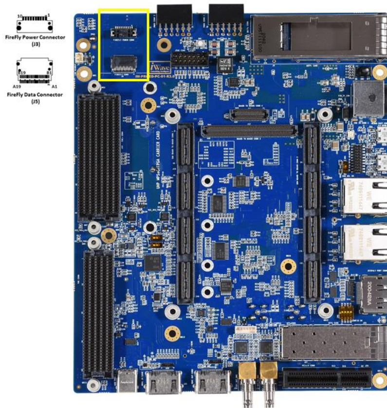
Figure 20 FireFly Connector
