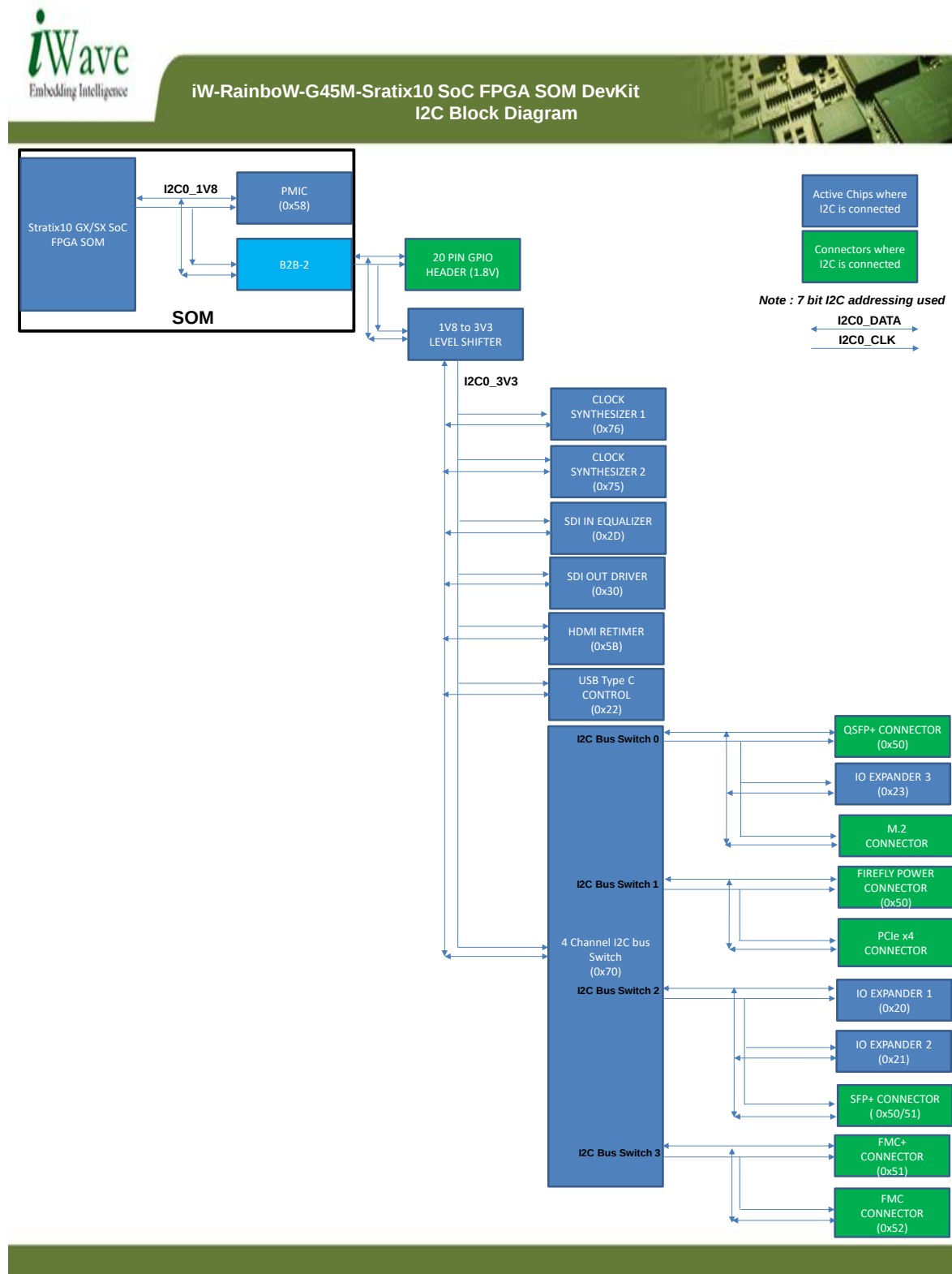
Figure 29 I2C Tree
