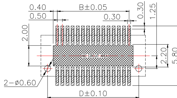
RECOMMENDED PCB PATTERN DIM.
