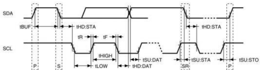
Figure: Bus timing requirements sequence
