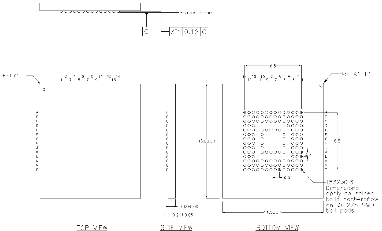
Figure 3.2-1. Package Dimension
