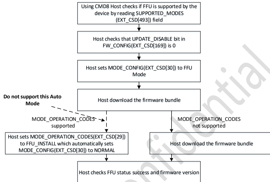
Figure 4.6-1. FFU Flow
