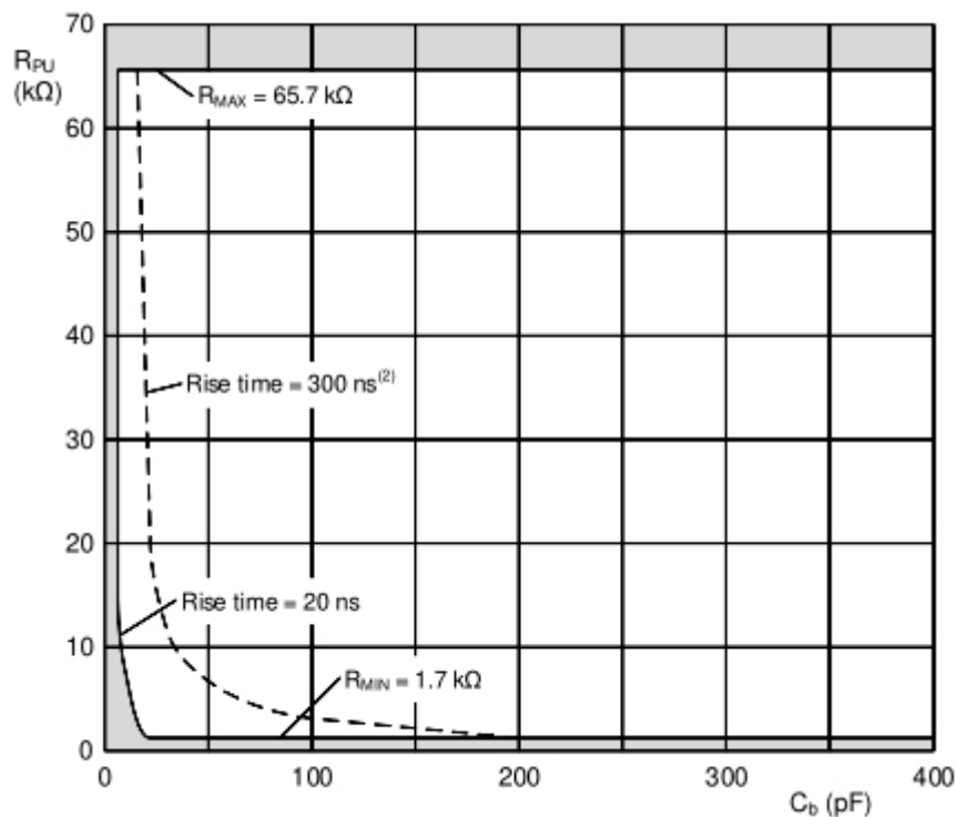
Figure 7.5 Bus requirements for 5V systems
