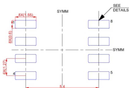
LAND PATTERN EXAMPLE(mm)
