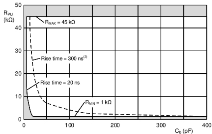
Figure 7.4 Bus requirements for 3.3V systems
