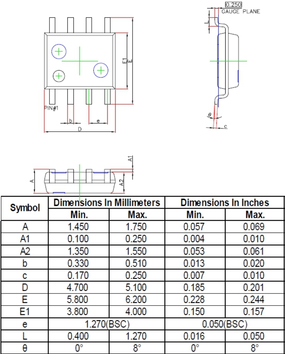
Figure 9.3 Package outline for SOP8
