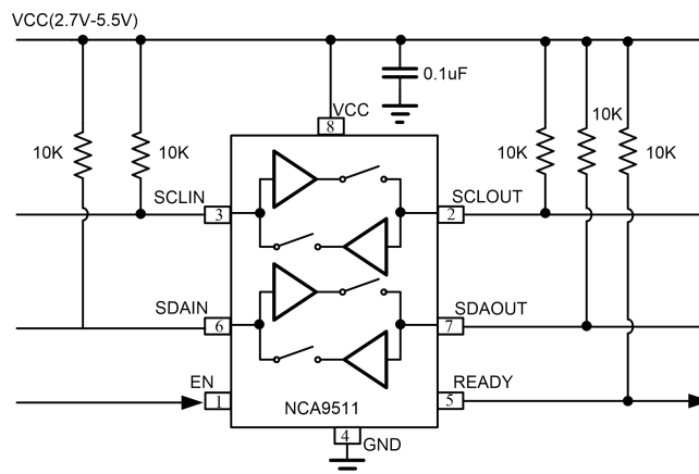
Figure 7.1 Typical application
