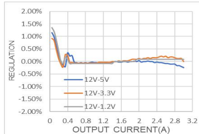
Load Regulation
