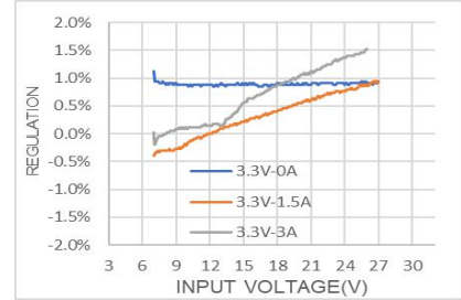
Line Regulation
