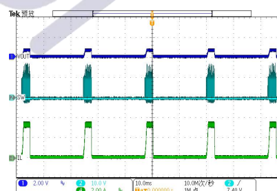
Output Short
