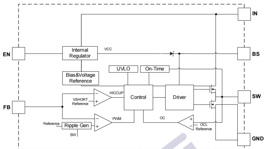
Block Diagram
