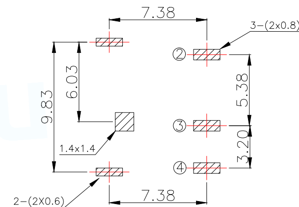
PCB.WELDING DRAWING (TOLERANCE:±0.05)
