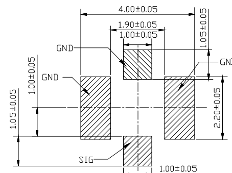
RECOMMENDED PCB LAYOUT 2 (GENERAL TOLERANCE IS ±0.05)
