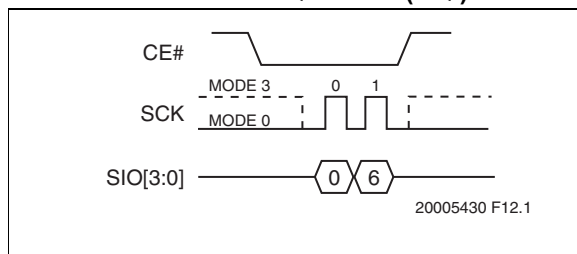
FIGURE 5-38: WRITE-ENABLE SEQUENCE (SQI)
