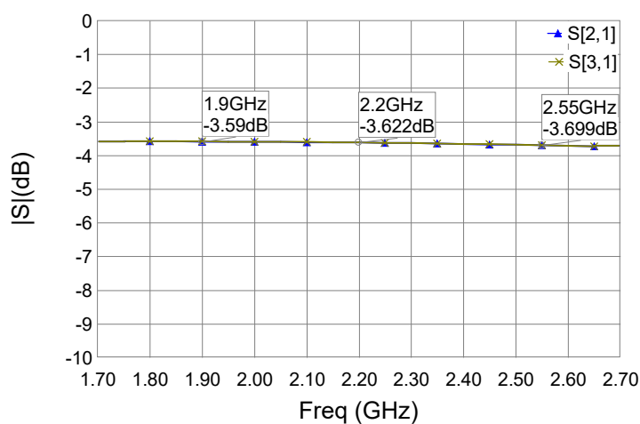
Figure 3. MPD1727W2/S2 Insertion Loss
