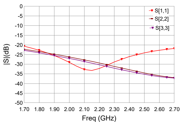
Figure 4. MPD1727W2/S2 Return Loss
