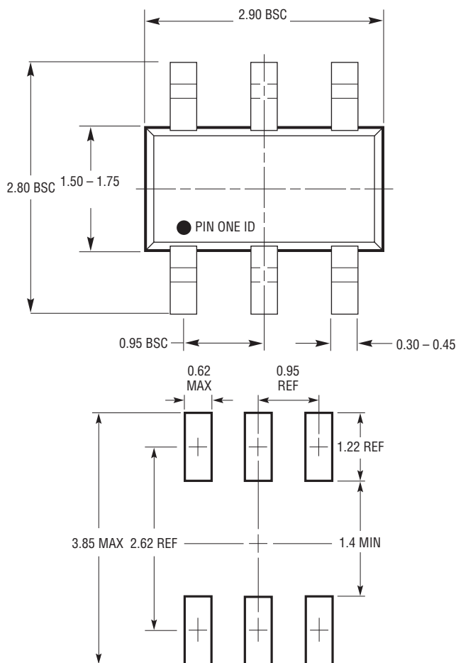
Figure 9. MPD1727S2 Outline Drawing and Recommended PCB Layout
