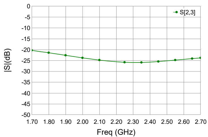
Figure 5. MPD1727W2/S2 Isolation
