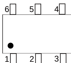
Figure 1. MPD1727W2/S2 (Top View)
