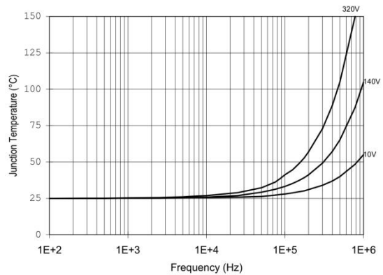
Figure 28. XL2110/XL2113 T_J vs. Frequency (IRFBC20) R_{GATE} = 33\Omega , V_{CC} = 15V
