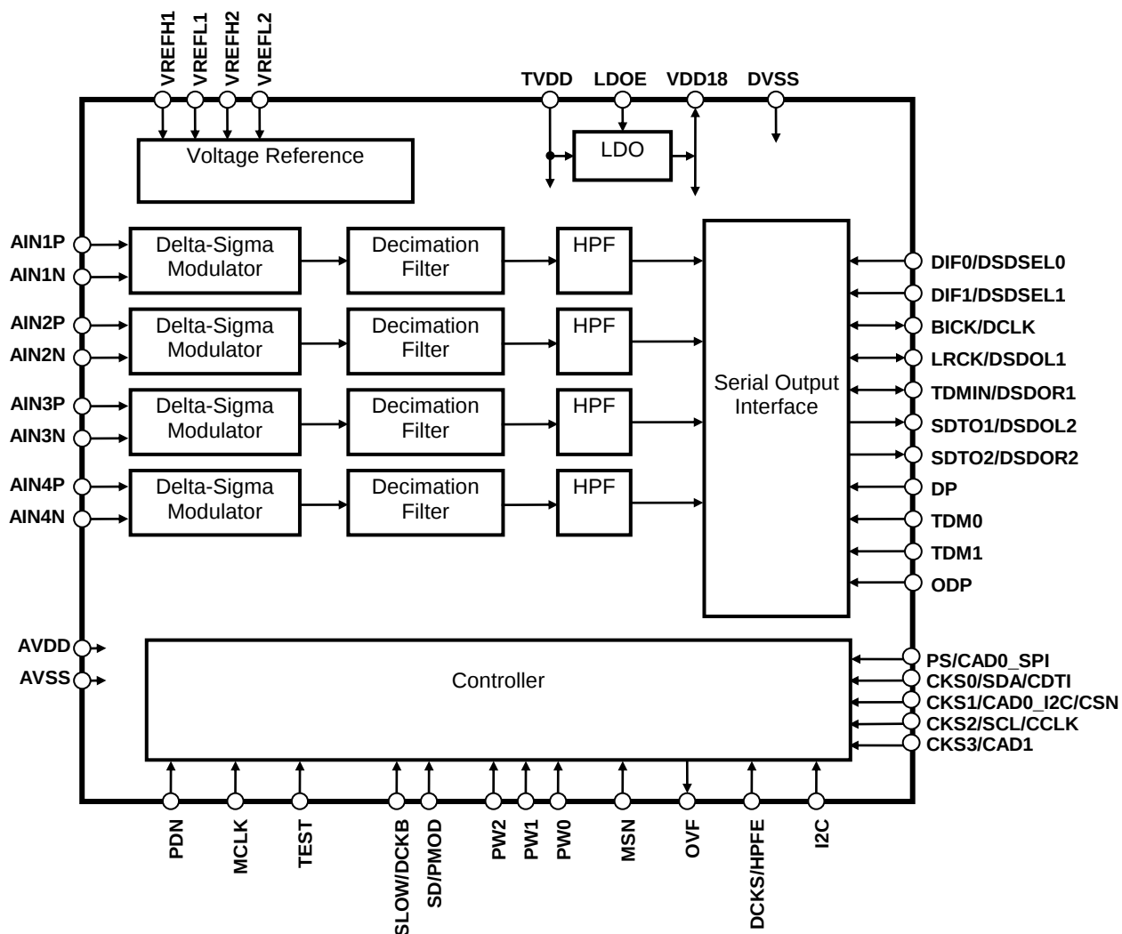
Figure 1. Block Diagram
