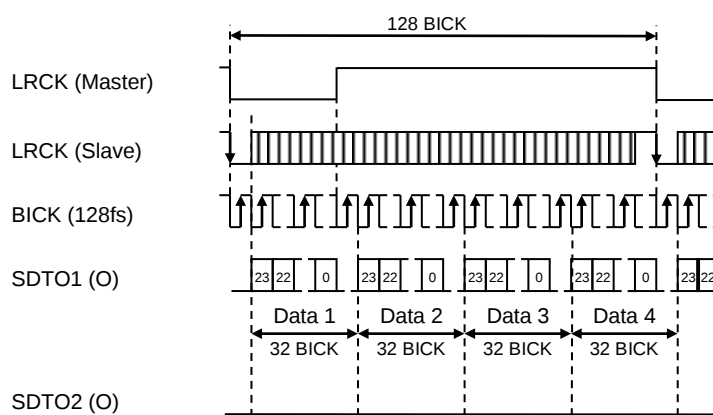
Figure 43. Mode 25/29 Timing (TDM128 mode, I²S Compatible)
