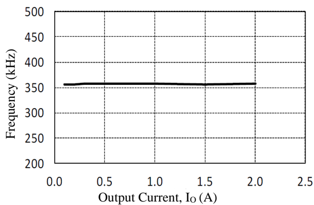
Figure 5-16. Operating Frequency
