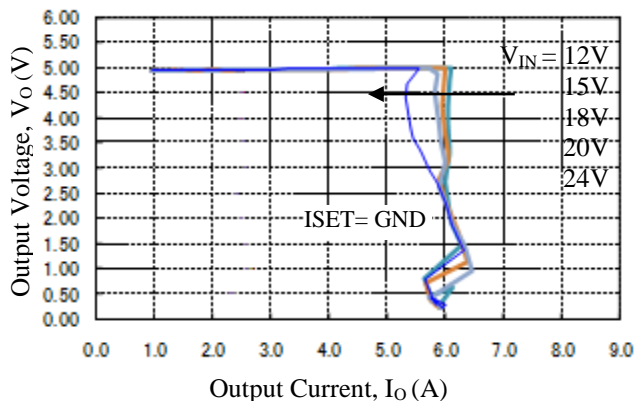
Figure 5-4. Overcurrent Protection
