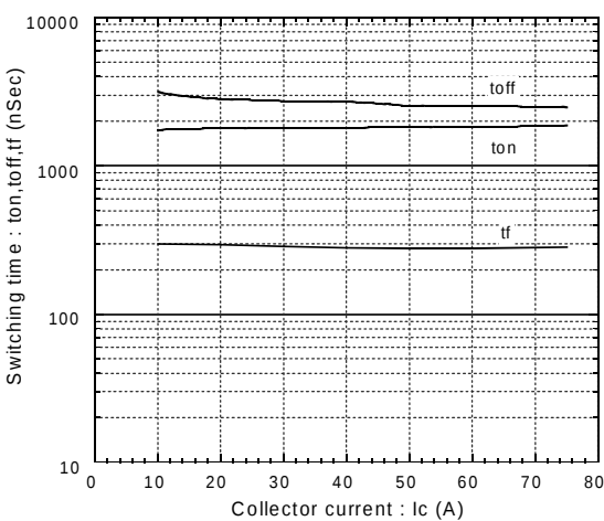
Switching time vs. Collector current Edc=600V,Vcc=15V,Tj=125°C
