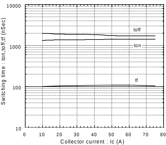
Switching time vs. Collector current Edc=600V,Vcc=15V,Tj=25°C
