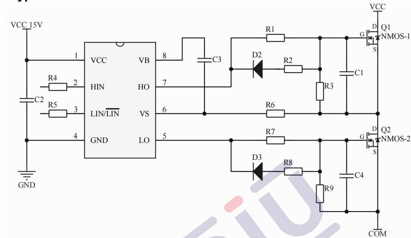
Typical application
