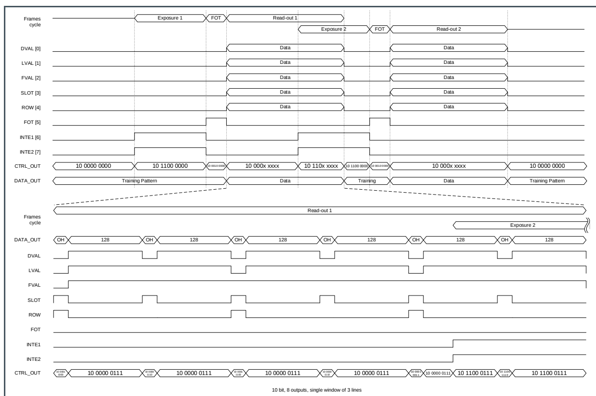
Figure 51: Detailed Timings of the Control Channel (8 outputs, 3 lines window)
