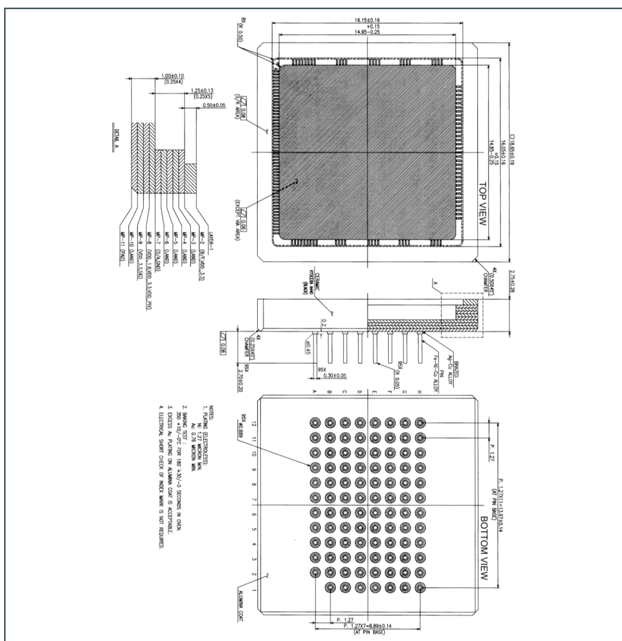
Figure 100: \mu PGA Package Drawing
