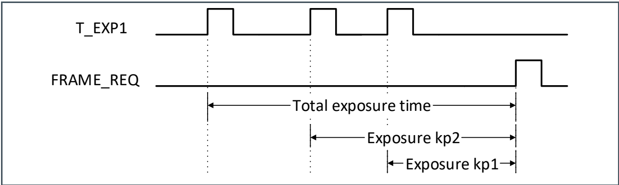
Figure 62: Timing of External Exposure Mode
