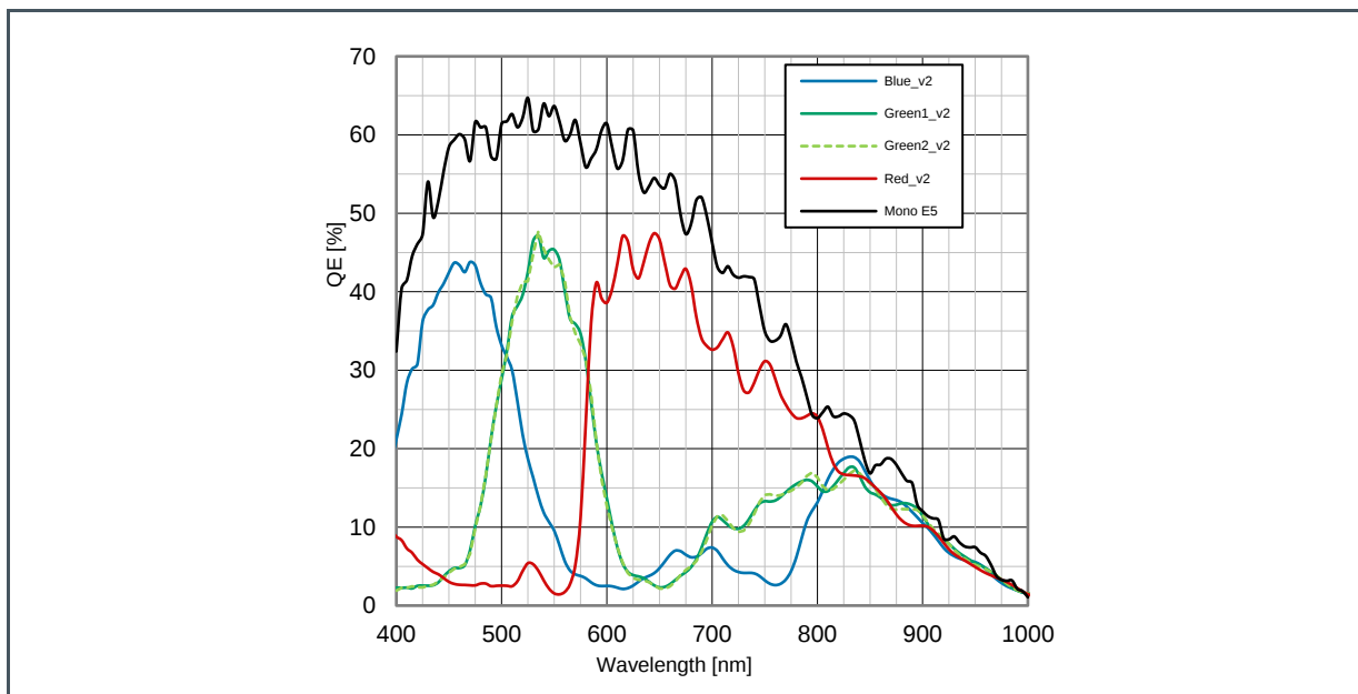
Figure 10: Typical Spectral Response of CMV4000 with RGB Color Filters and D263 Cover Glass and Mono
