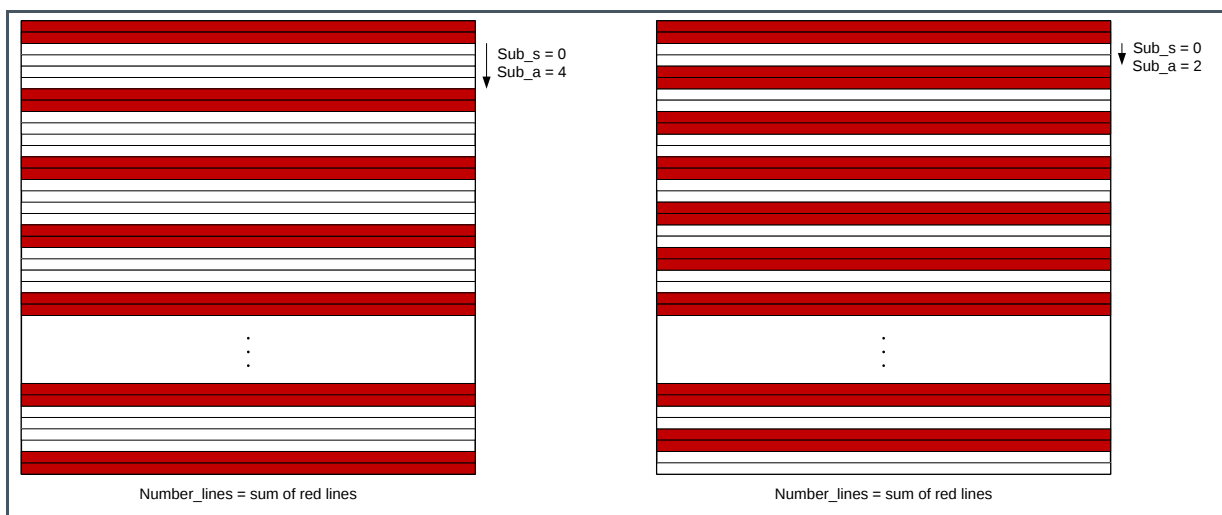
Figure 73: Subsampling Examples in Advanced Mode (skip 4x and skip2x)
