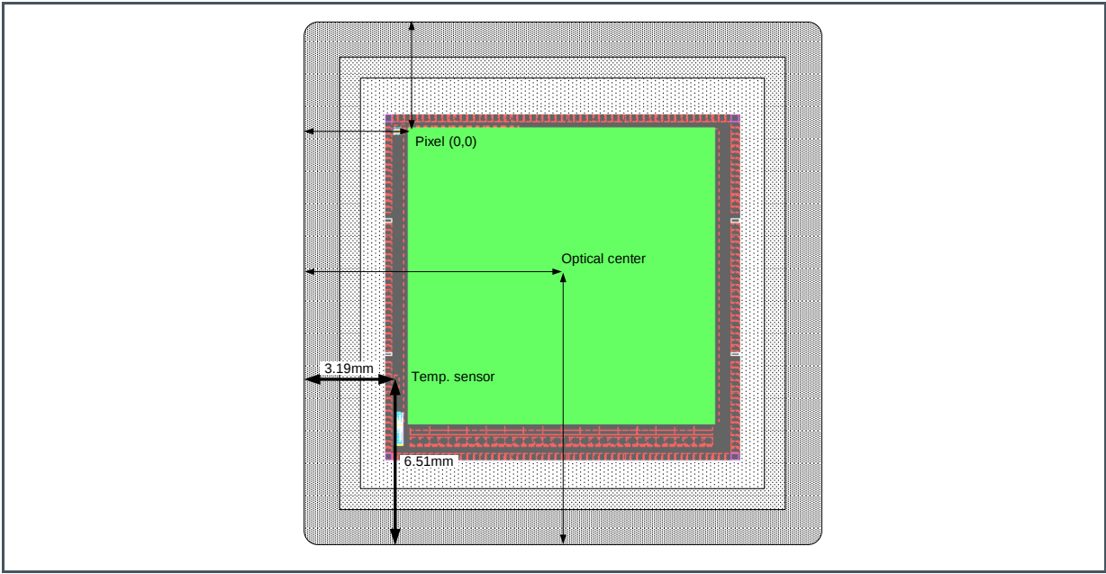
Figure 14: Location of the Temperature Sensor
