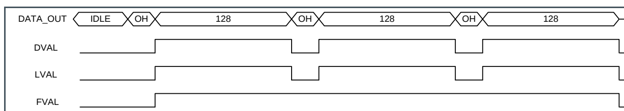
Figure 49: DVAL, LVAL and FVAL Timing in 16 Outputs Mode
