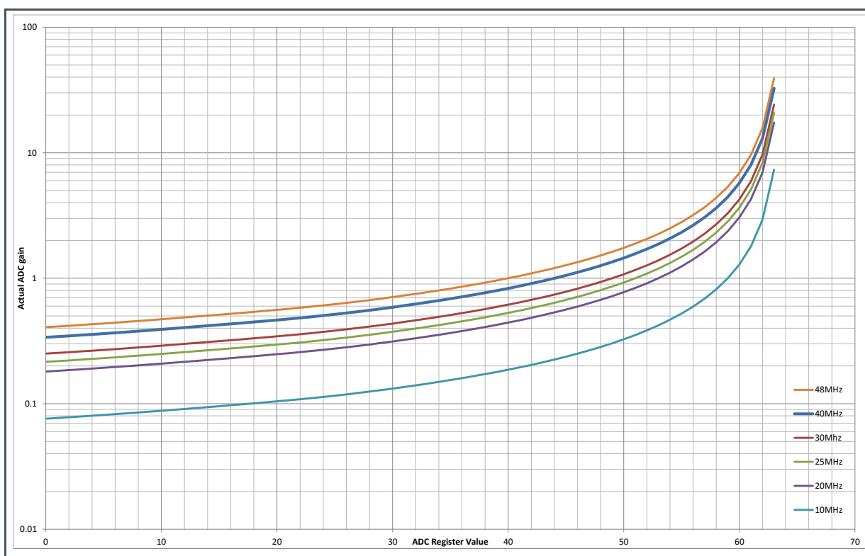
Figure 85: Typical Graphs of Gain Setting
